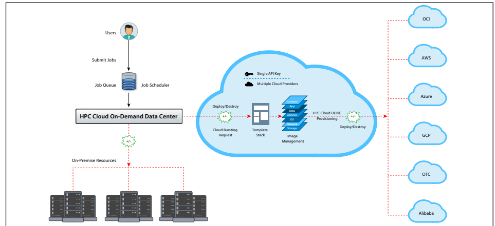
The ODDC gives immediate access to all on-premise as well as cloud compute resources.
